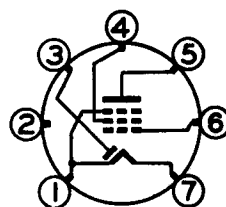
RTMA 6AU BOTTOM VIEW
